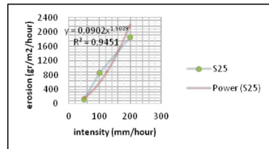
Figure 4: Regression graph of soil erosion for the slope of 25°
