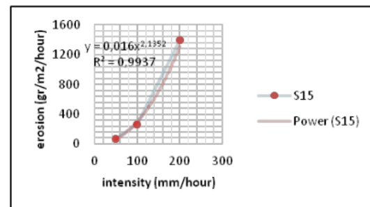
Figure 3: Regression graph of soil erosion for the slope of 15°
