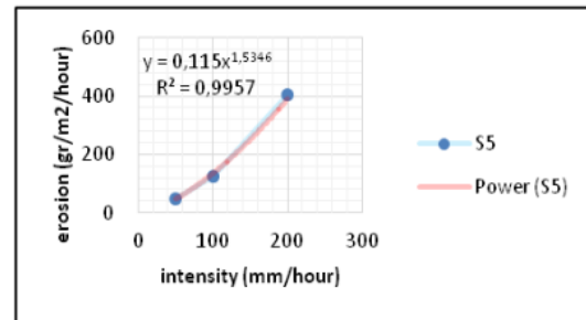
Figure 2: Regression graph of soil erosion for the slope of 5°
