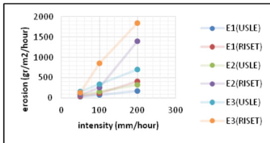
Figure 1: The graph of soil erosion comparison between USLE model and the experiments
